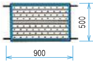
L09PC (7.4kg) HPF布板09PC
