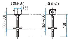
ON35×450P (5.5kg) (ON3545)
