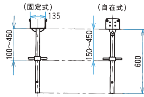
ON35×600P (6.3kg) (ON3560)
